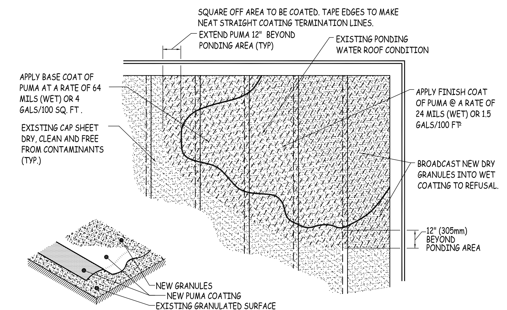
LOCALIZED PONDING & PUMA COATING DETAIL
